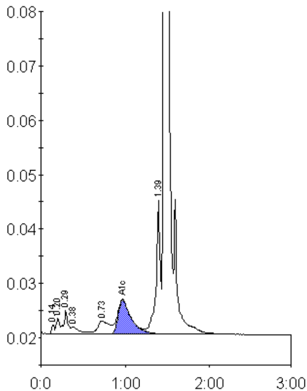
Peak table - ID: 10526799
